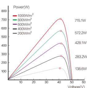
Power-Voltage Curve ( 715W ) Cells temp.=25°C
