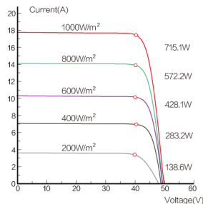
Current-Voltage Curve ( 715W ) Cells temp.=25°C
