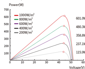
Power-Voltage Curve (600W) Cells temp.=25°C
