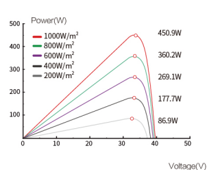
Power-Voltage Curve ( 450W ) Cells temp.=25°C
